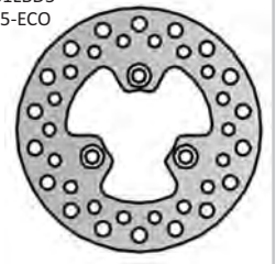
NG1022 Ø190xØ58x3,7 4 IN 1 MULTI DISC
